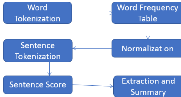
Fig.2: Algorithm For Summarization
